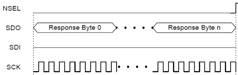
Figure 5. SPI Read Command—Clock Out Read Data
