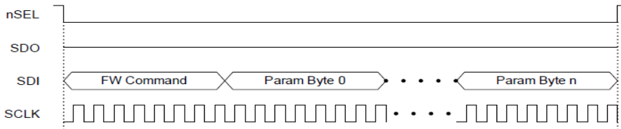
Figure 3. SPI Write Command
