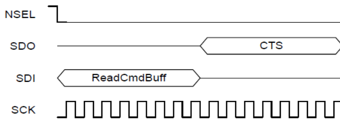
Figure 4. SPI Read Command—Check CTS Value
